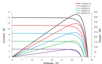
I-V/P-V Curve at Different Irradiation SS8-54HD-425N
